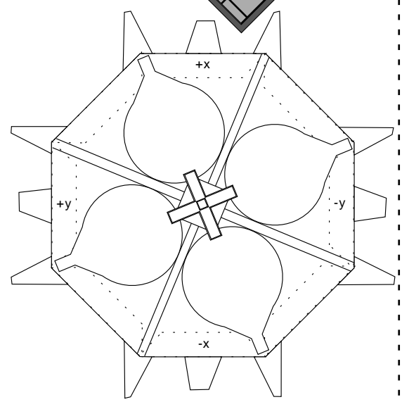
Bottom (-Z) panel piece -- inside
