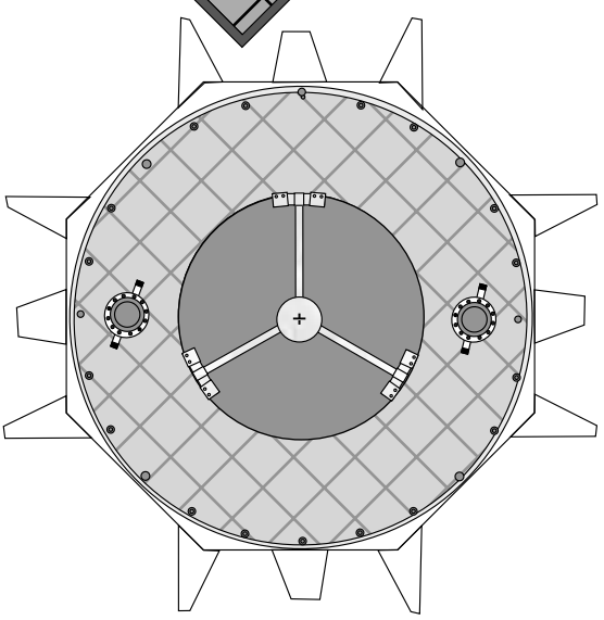
Bottom (-Z) panel piece -- outside
